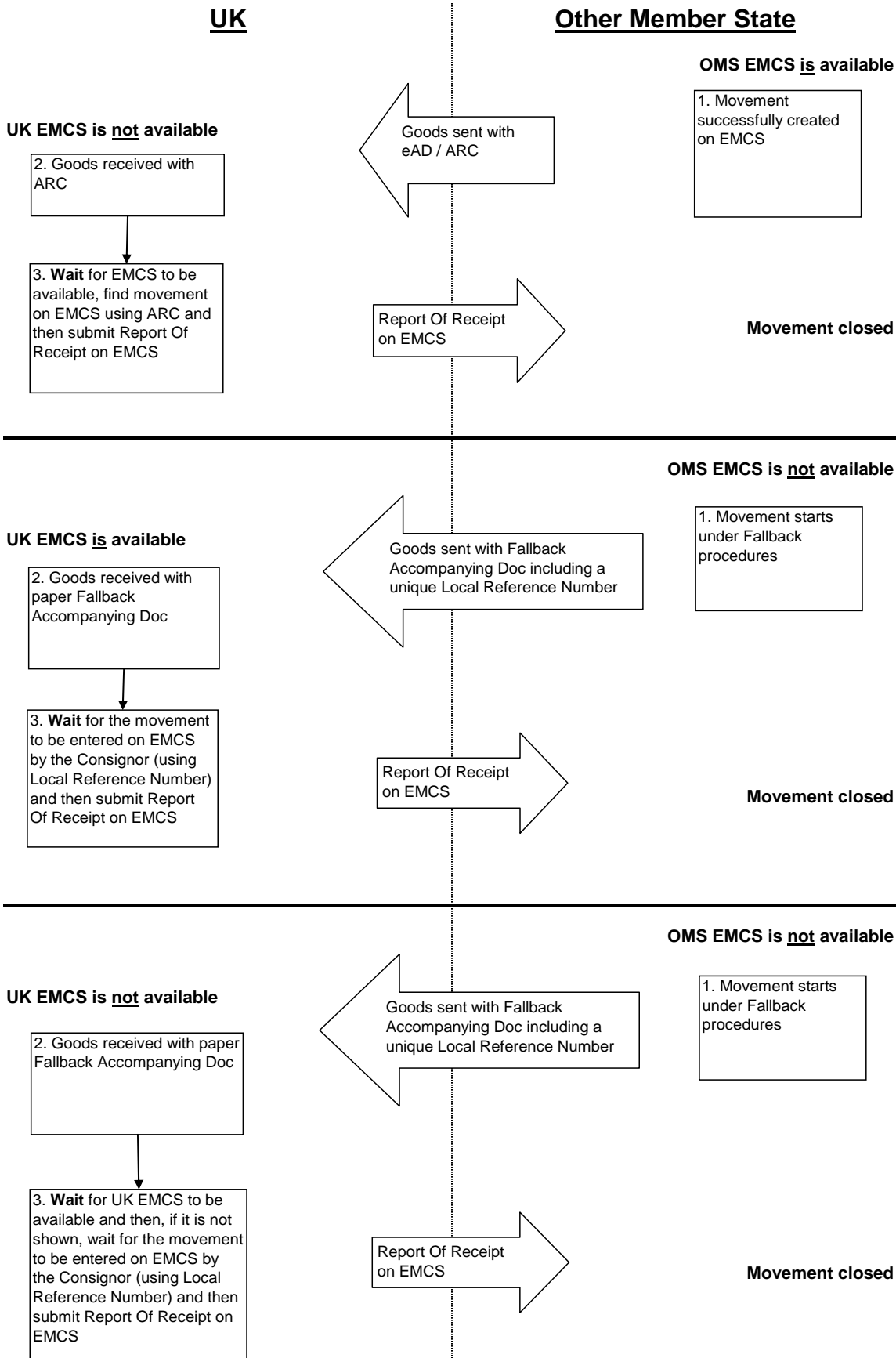
Figure 4 Submitting a Report of Receipt (ROR) in fallback
